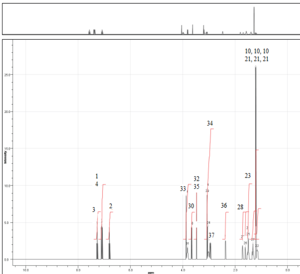
Figure 47: Better resolution of 1 H-NMR spectrum of (AZ-4) by Marvin Sketch.
